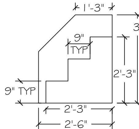
3 STAIRS - NOTE BUILD 1 J2 SIDE VIEW - SCALE: \frac{1}{2}'' = 1'-0''
