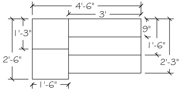
1 STAIRS - NOTE BUILD 1 J2 TOP VIEW - SCALE: \frac{1}{2}'' = 1'-0''
