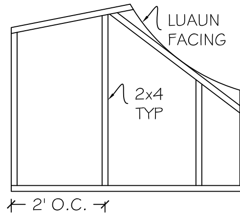
2 PLATFORM FRAMING - NOTE BUILD 1 J1 GROUNDPLAN VIEW - SCALE: 1/2" = 1'-0"
