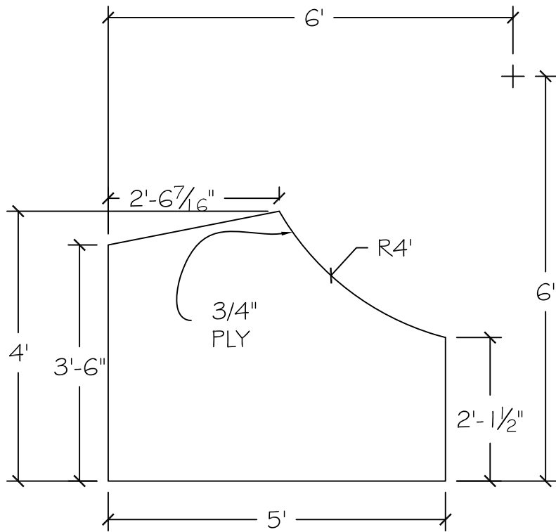
1 PLATFORM - NOTE BUILD 1 J1 GROUNDPLAN VIEW - SCALE: 1/2" = 1'-0"
